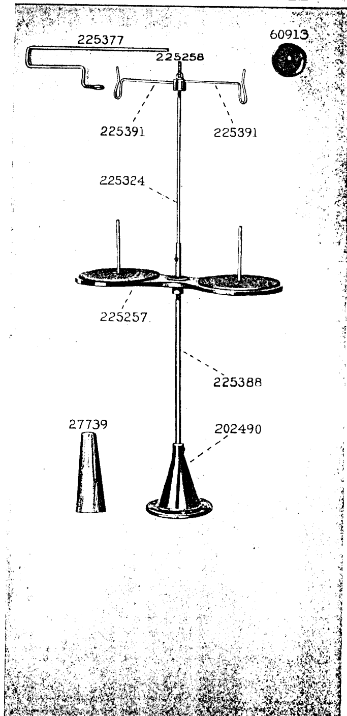
PLATE 14363—ONE-SIXTH SIZE
